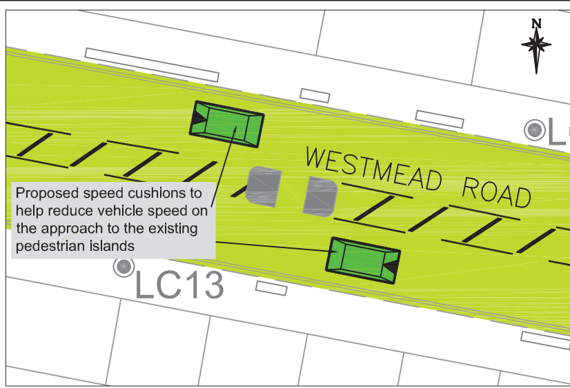
TYPICAL SPEED CUSHIONS DETAIL
