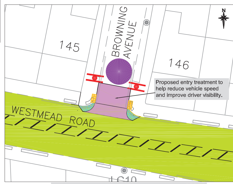
TYPICAL RAISED ENTRY TREATMENT DETAIL
